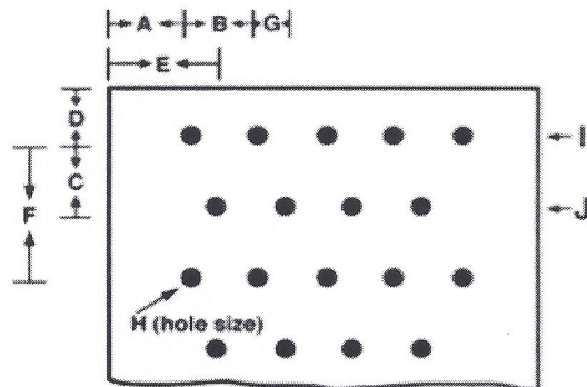
2 Staggered Pattern
